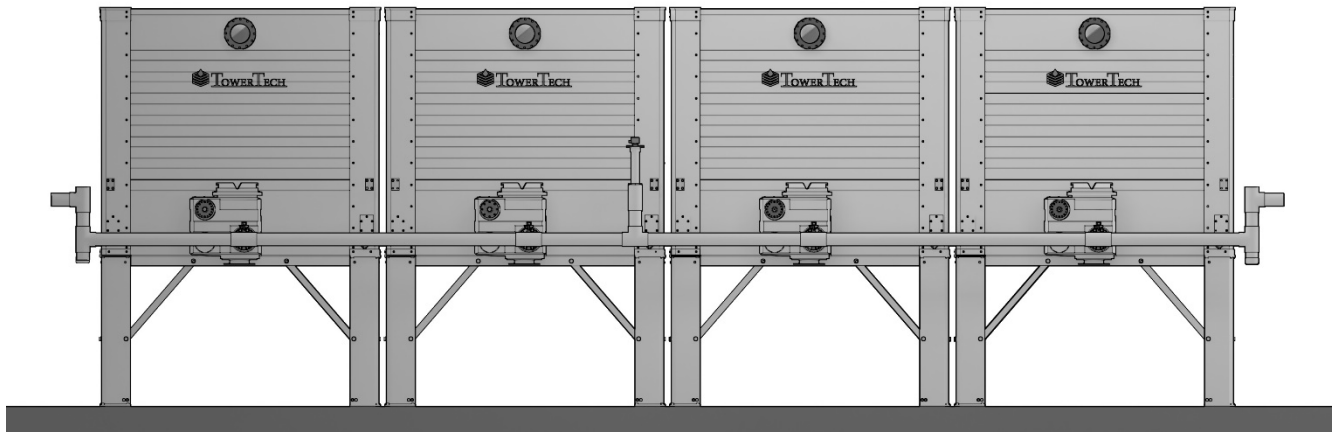
Figure 40 – Typical Overflow/Equalization Piping for large tower installations with Electronic Level Control.
