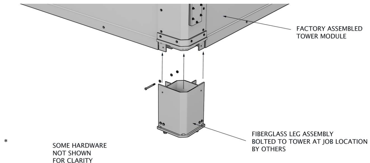
Figure 30 – Installation Detail for 1' Sub-Structure
