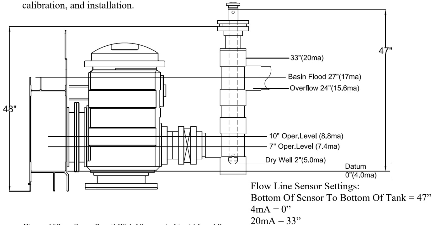
Figure 18B – Sump Detail With Ultrasonic Liquid Level Sensor
