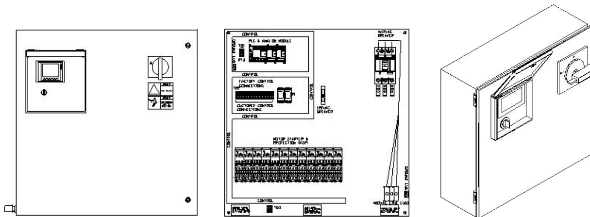
Figure 15 – Typical Motor Control Panel for 10-Fan Cooling Tower Module. (VIEWSCREEN® touch screen standard on all Tower Tech T9900 control panels ordered after August 31, 2011.)
