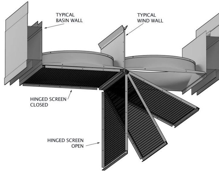
Figure 55A – Opening Full Screen Fan Guard
