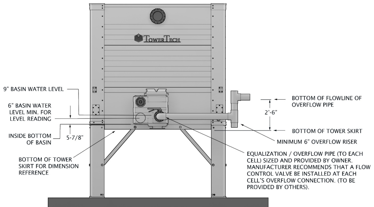
Figure 19A – Equalization/Overflow Pipe Detail (No Ultrasonic Level Sensor)
