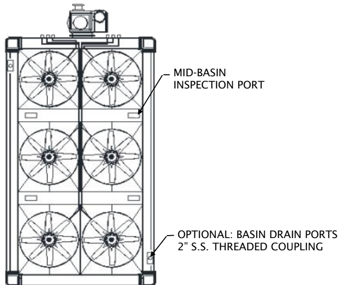
Figure 47 – Mid-Basin Inspection Ports (6-fan tower module shown)
