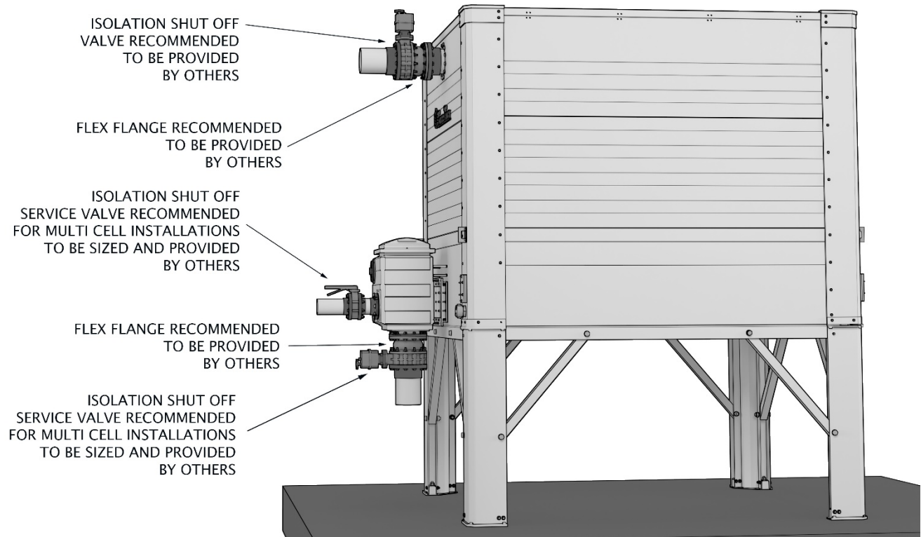
Figure 37 – Connection Flexible Flanges & Flow Control Valves
