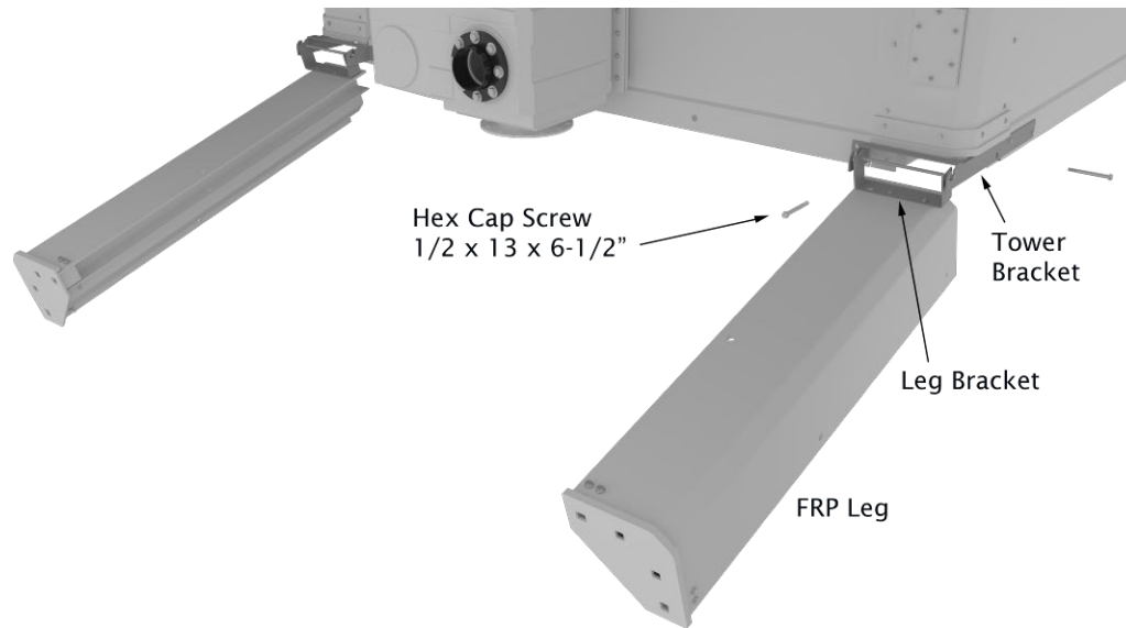
Figure 22 – Folding Leg Bracket Detail
