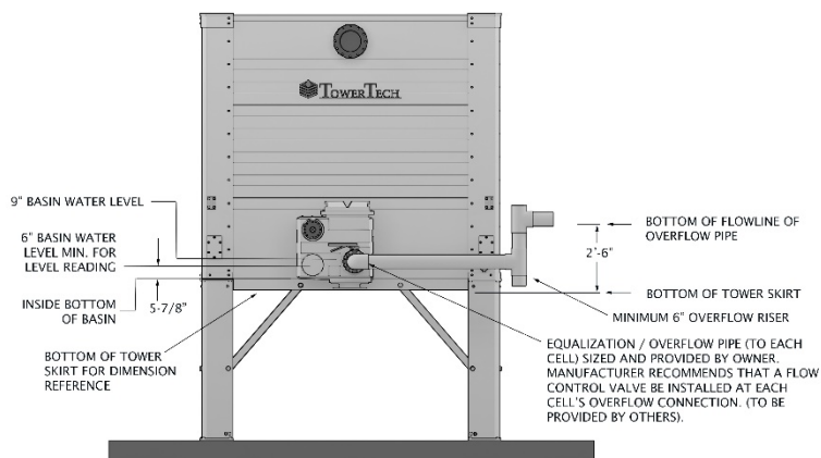
Figure 39A – Typical Overflow/Equalization Pipe
