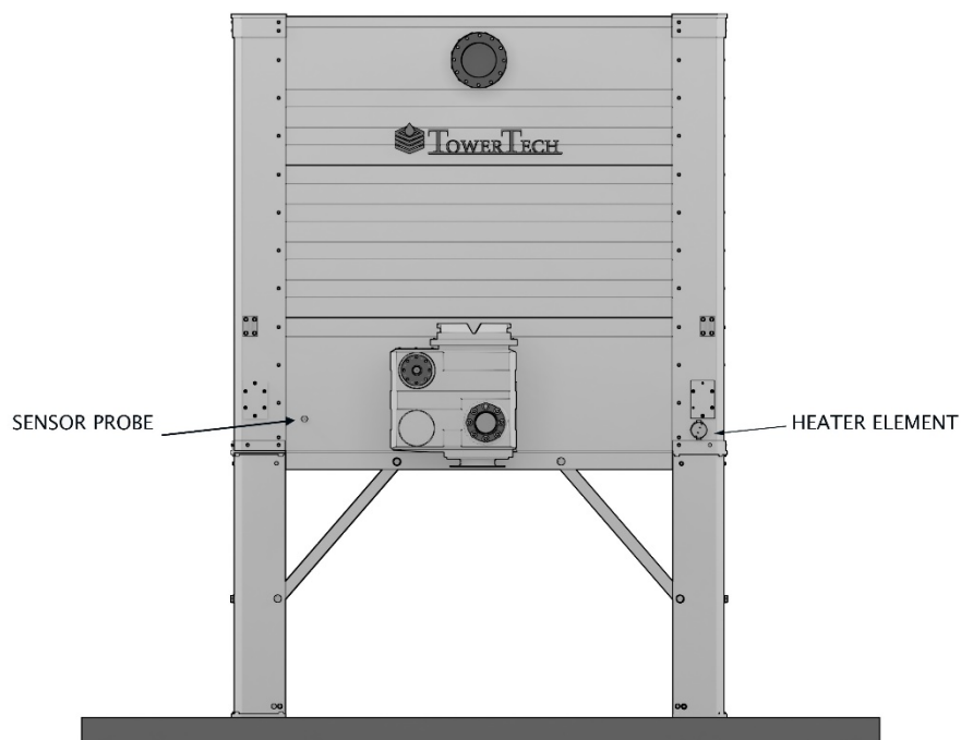
Figure 17 – Immersion Basin Heater and Sensor Probe Location
