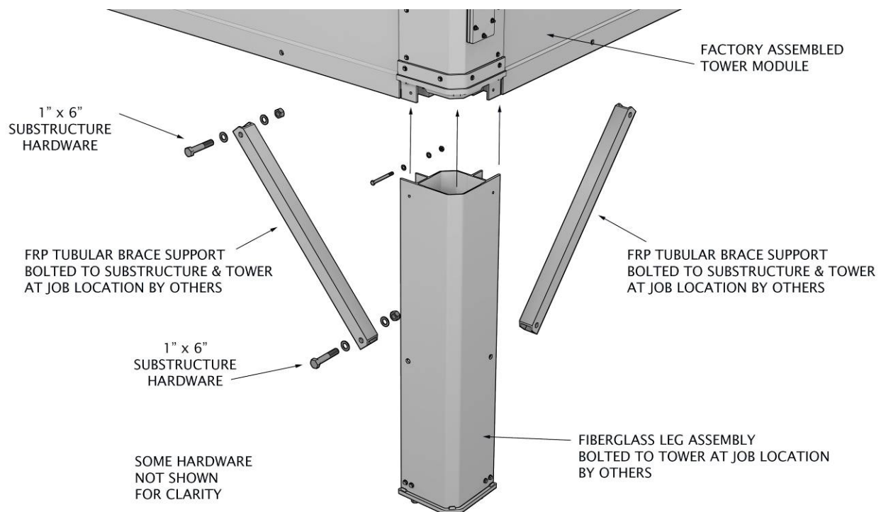
Figure 29 – Installation Detail for Sub-Structures Taller Than One Foot (30.5 cm)
