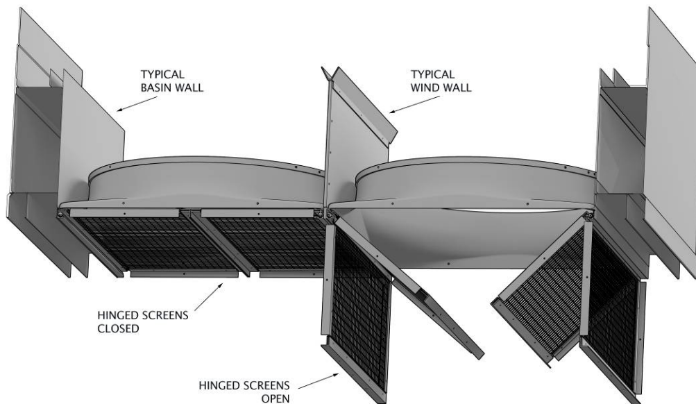
Figure 55B – Opening Split Screen Fan Guard
