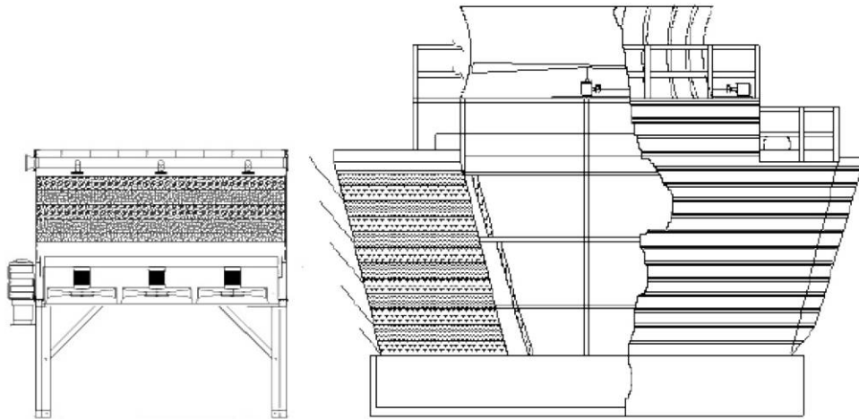
Figure 2 – TTXL versus Conventional Induced-Draft Cross-Flow Tower
