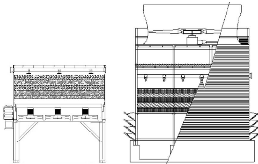
Figure 3 – TTXL versus Conventional Induced-Draft Counter-Flow Tower
