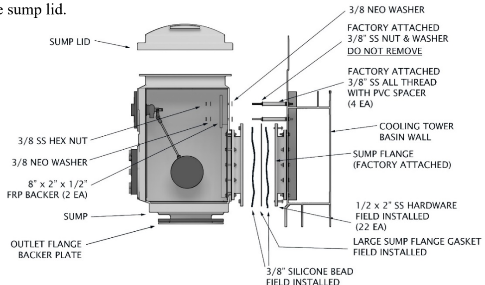
Figure 35 – Sump Installation Detail
