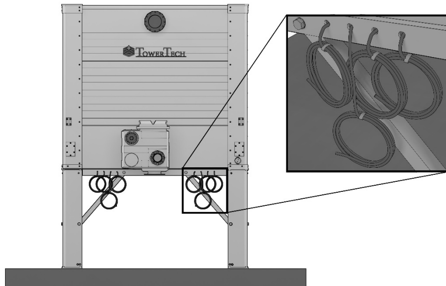
Figure 13C – Pre-wire to Pigtails
