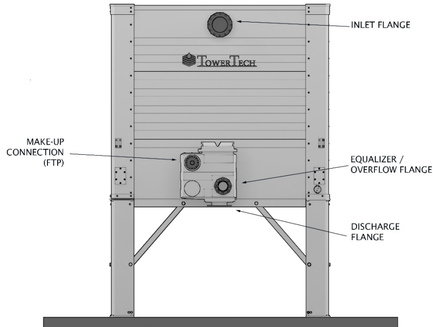
Figure 36 – Standard Piping Connections
