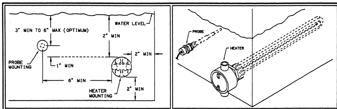
Figure 49 – Location of Basin Heater Probe & Element
