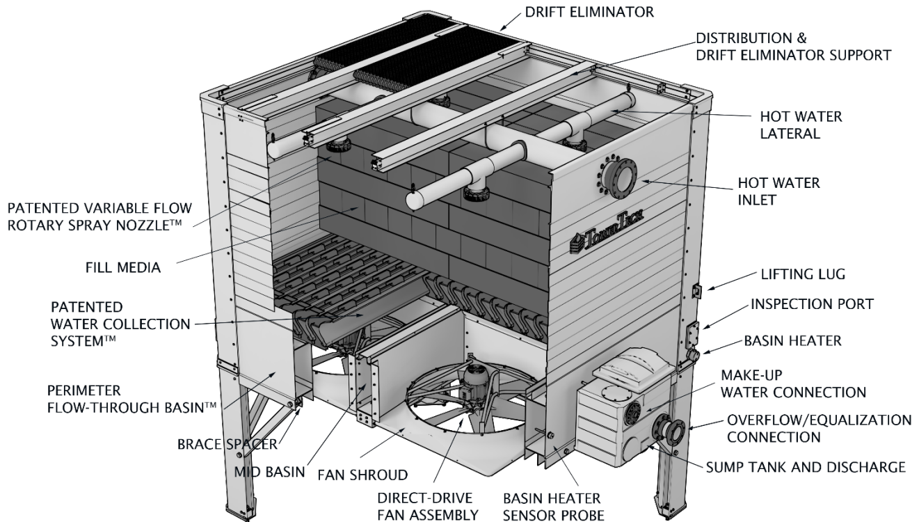
Figure 1 - TTXL 3-D Cut-Away View
