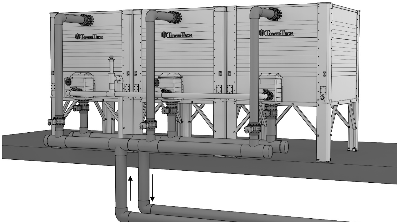
Figure 21 – Multi-Tower Layout and Piping Recommendations
