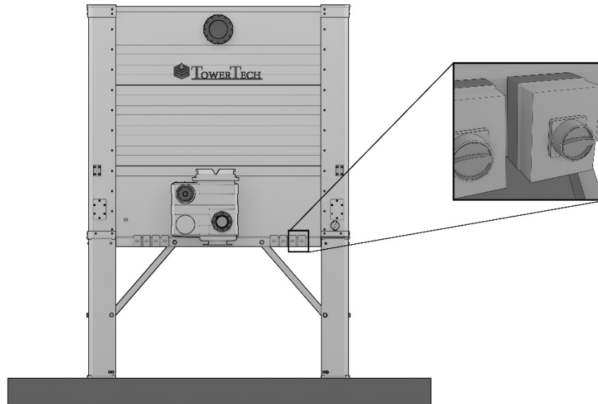
Figure 13B – Optional Rotary-Type NEMA 4X Lockout Disconnect Switches
