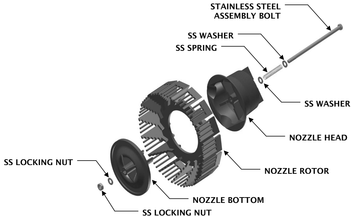
Figure 53 – Exploded View of Rotary Spray Nozzle
