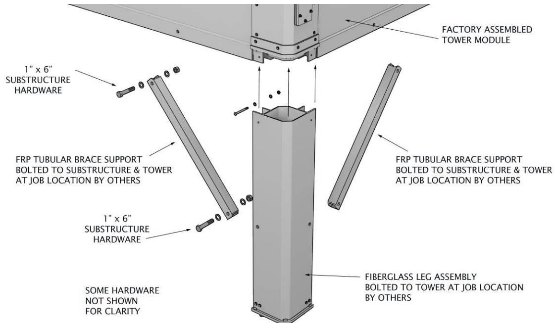
Figure 14 – Tower Sub-Structure
