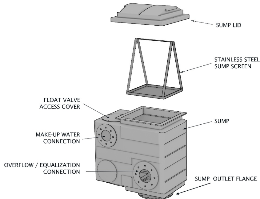
Figure 57 – Sump Layout, Sump Screen Detail
