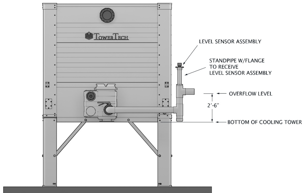
Figure 18A – Ultrasonic Liquid Level Sensor Location
