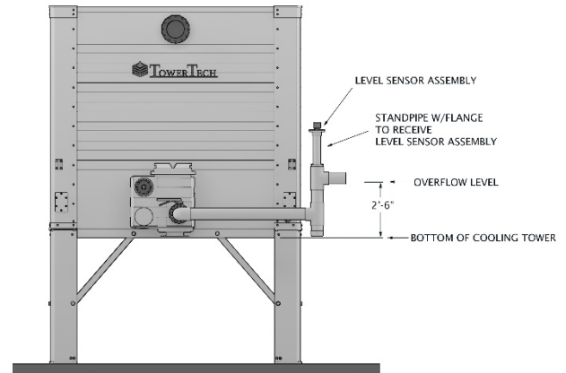
Figure 39B – Typical Ultrasonic Stand Pipe with Overflow
