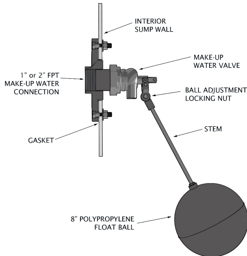
Figure 7 – Mechanical Float Valve
