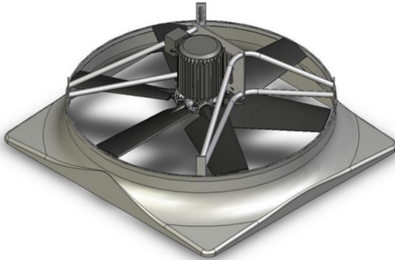
Figure 8 – Motor, Motor Support, Fan, Fan Shroud
