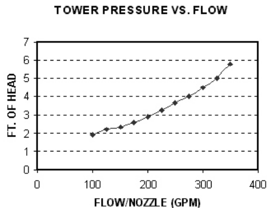
Graph 2 – Tower Pressure versus Flow
